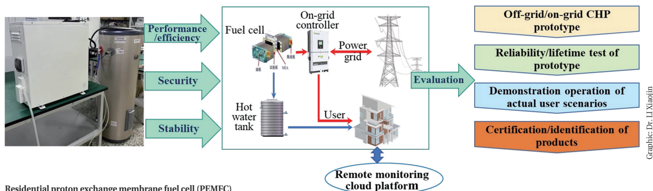
Residential proton exchange membrane fuel cell (PEMFC) cogeneration system.
